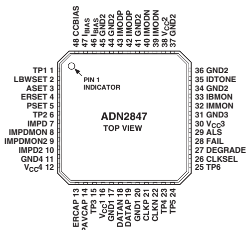
48-Lead LFCSP
