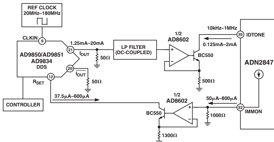
Figure 9. Application Curcuit to Allow Fiber Identification Using the AD9850/AD9851
