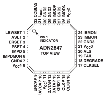
32-Lead LFCSP
