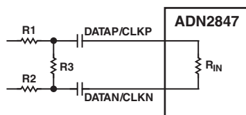
Figure 8. Attenuation Circuit
