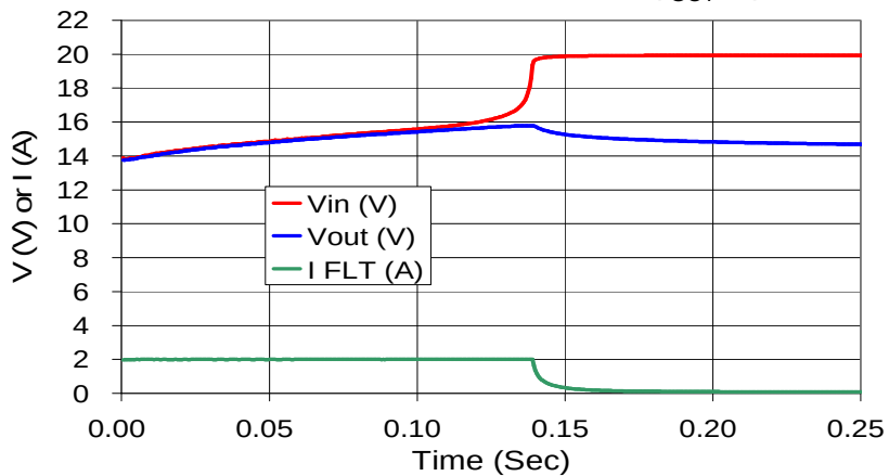
Typical Fault Response: ZEN132V230A16LS 20 V/2 A Current Limited Source ( I_{OUT}=0 )
