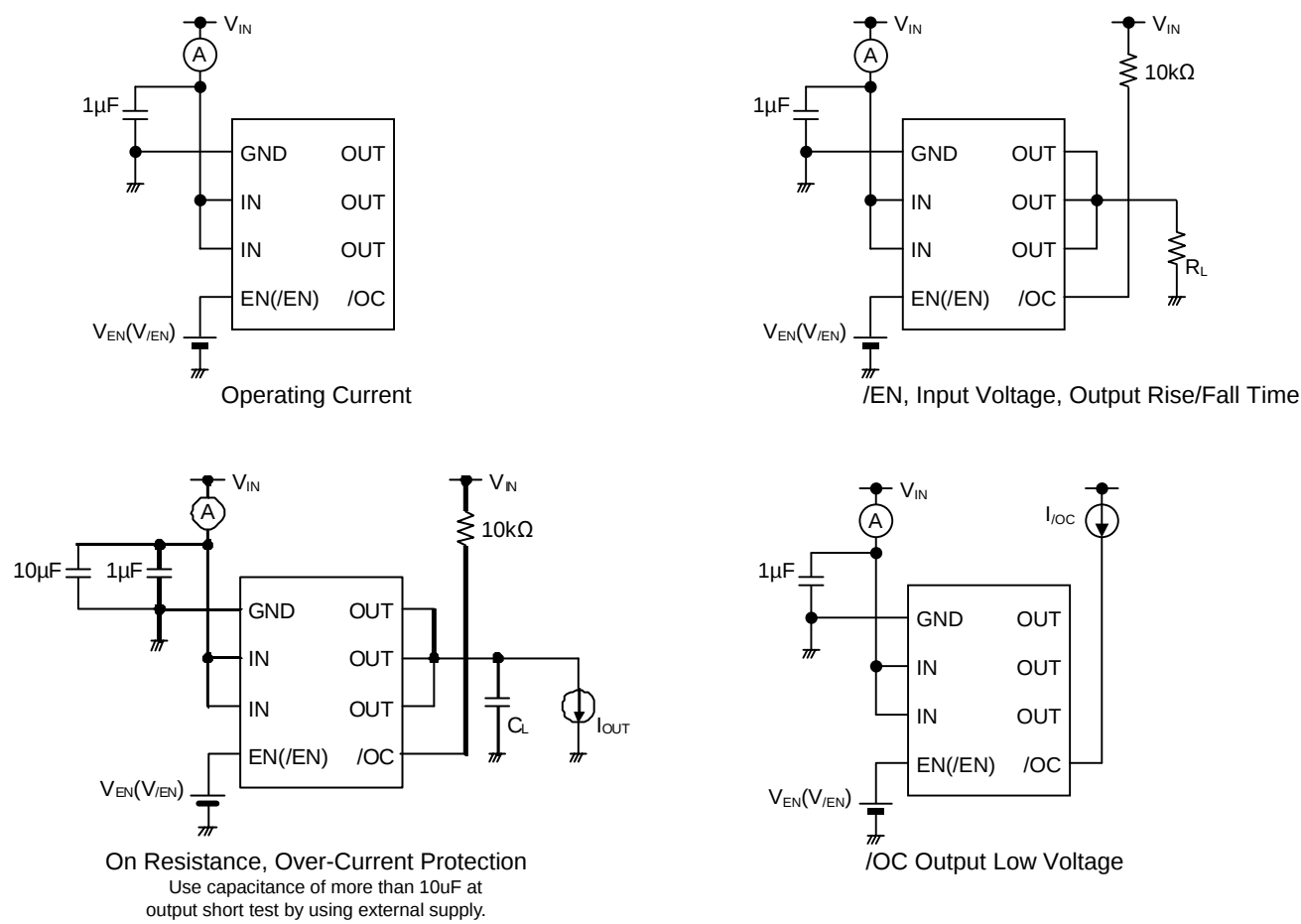
Figure 4. Measurement Circuit
