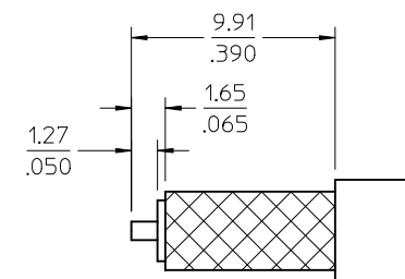
RECOMMENDED CABLE STRIP DIMENSIONS
