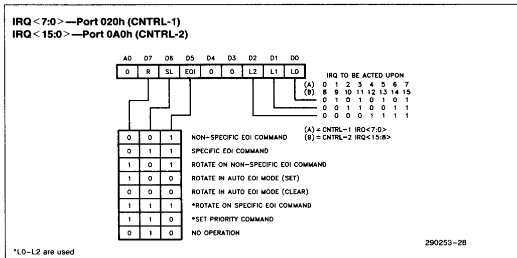
Figure 5-9. OCW2
