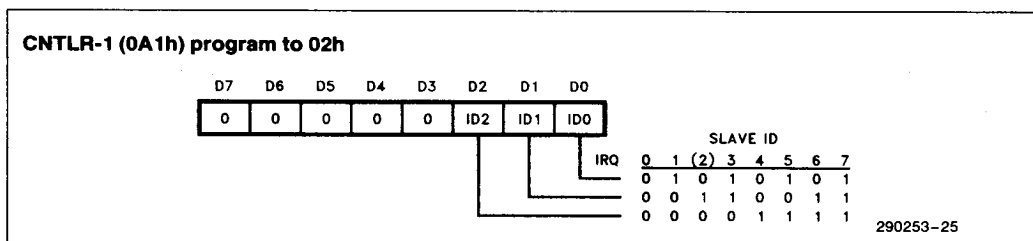
Figure 5-6. ICW3 (Slave Device)
