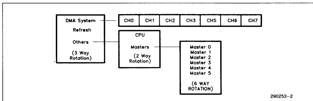
Figure 2-1. Arbitration Priority
