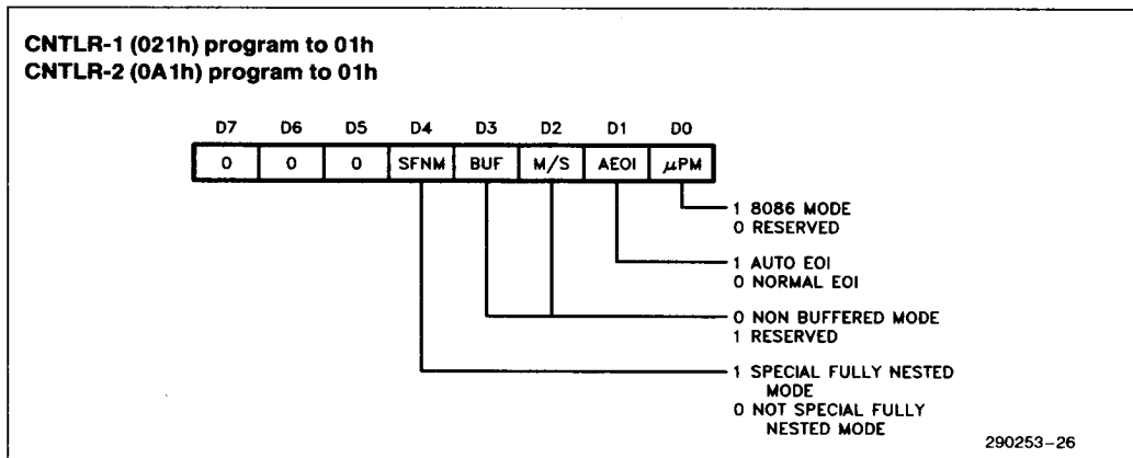
Figure 5-7. ICW4 021h(CNTLR-1) or 0A1h(CNTLR-2)
