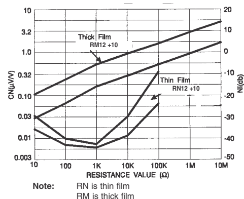
Current Noise
