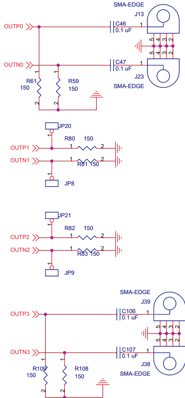
Figure 3. CDCLVP2102EVM—Schematic
