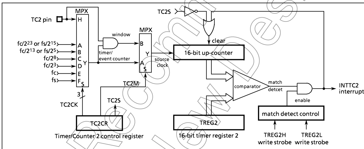
Figure 2-21. Timer/Counter 2 (TC2)
