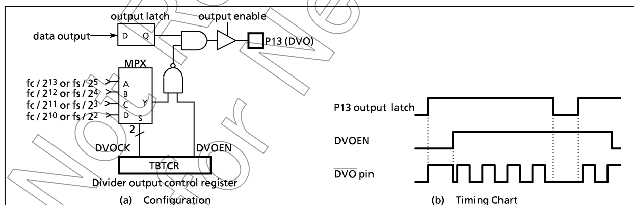
Figure 2-11. Divider Output
