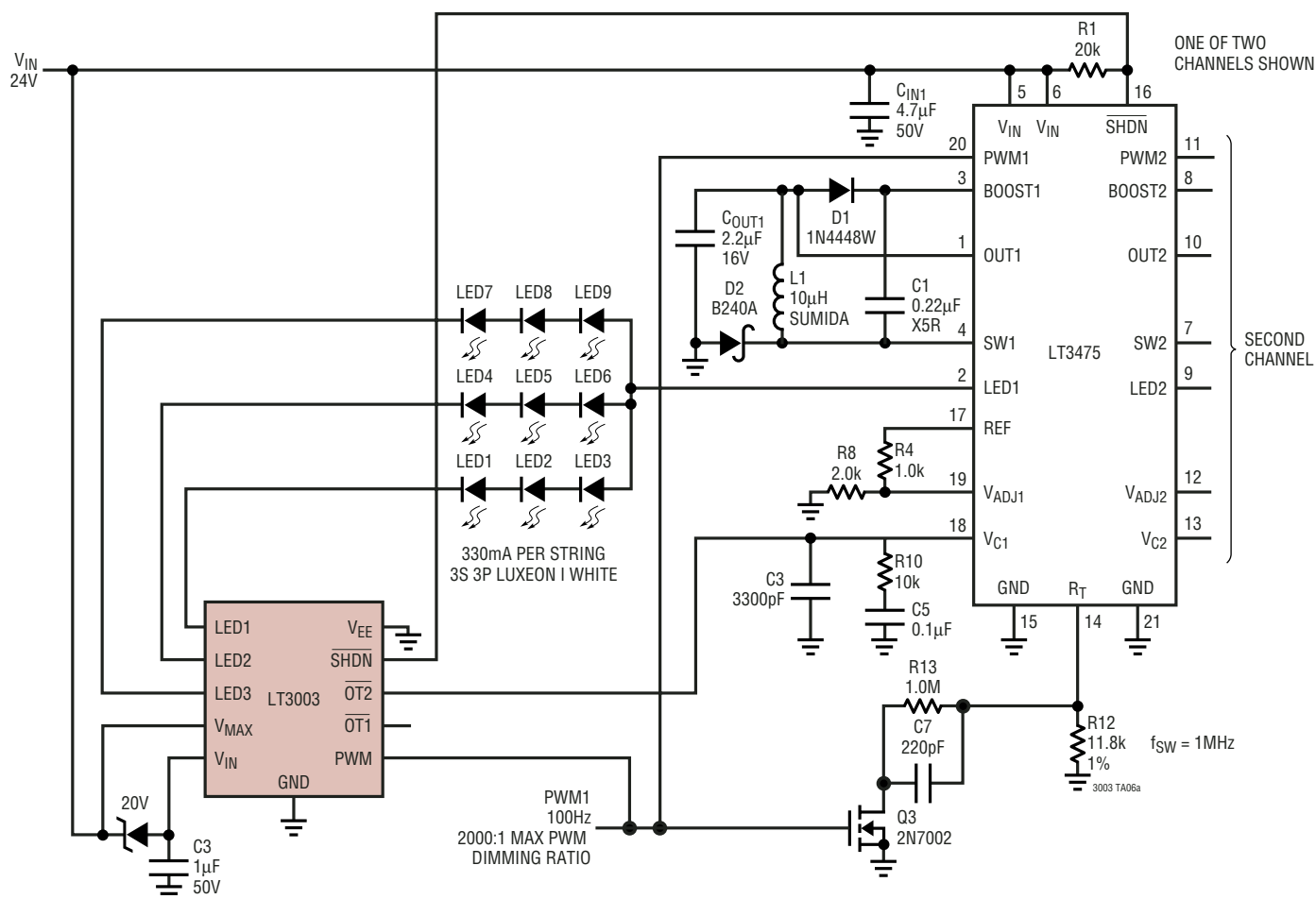
1A Buck LT3003 with the LT3475
