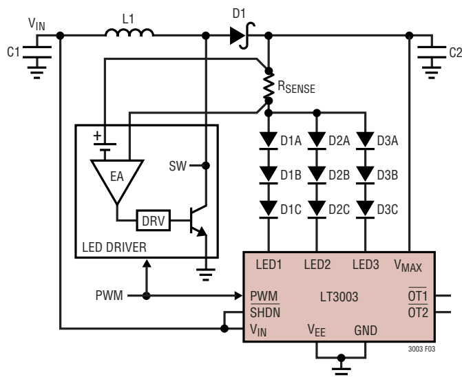
Figure 3. Boost Mode
