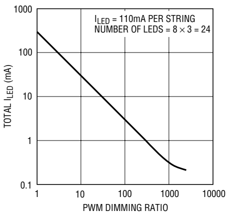
PWM Dimming
