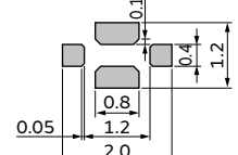
NFM18PS
