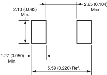
DO-214AA (SMB)
