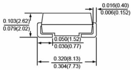
SMC/DO-214AB
