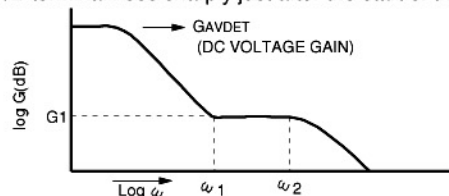
Fig.44 Gain-frequency characteristics between point B and point C shown in Fig.43
