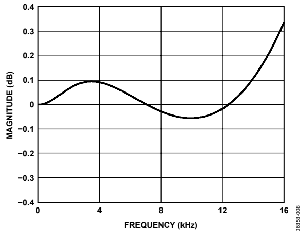
Figure 13. De-Emphasis Error, Audio Sampling Rate = 32 kHz
