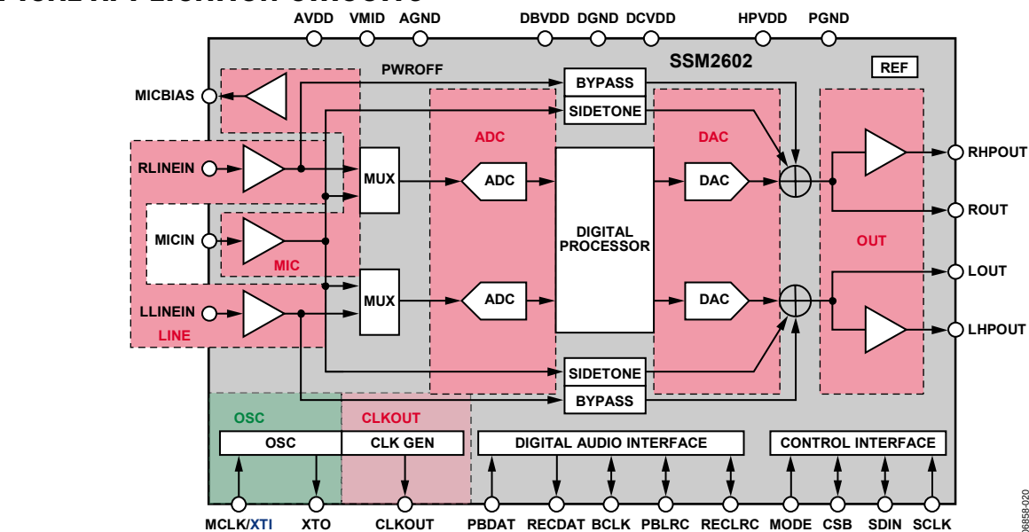
Figure 31. SSM2602 Power Management Functional Location Diagram (Control Register R6, Bit D0 to Bit D7)
