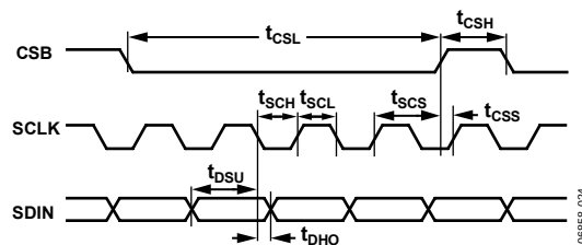
Figure 3. SPI Timing
