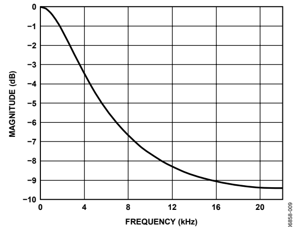
Figure 14. De-Emphasis Frequency Response, Audio Sampling Rate = 44.1 kHz
