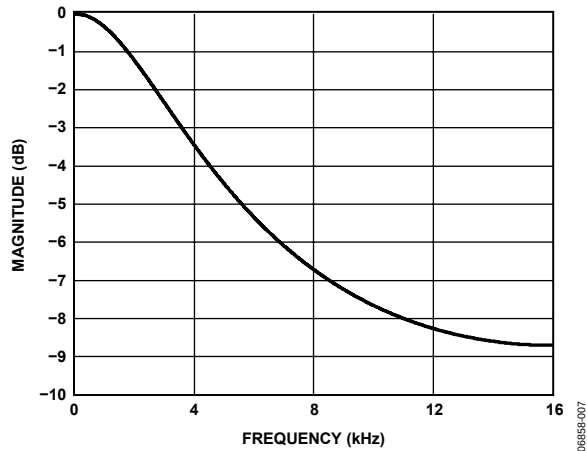
Figure 12. De-Emphasis Frequency Response, Audio Sampling Rate = 32 kHz
