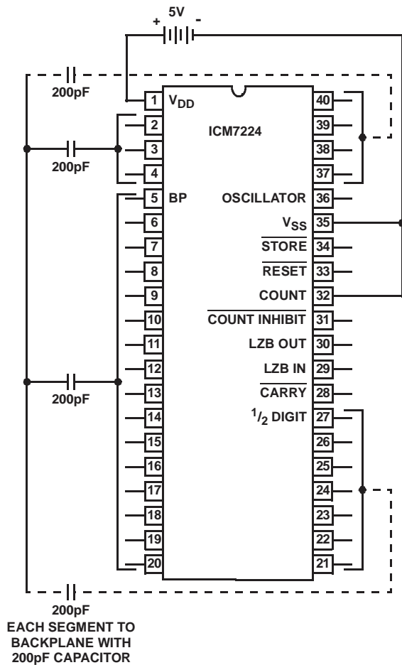
FIGURE 6. TEST CIRCUIT
