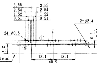
PCB mounting hole layout (Connector mounting side)
