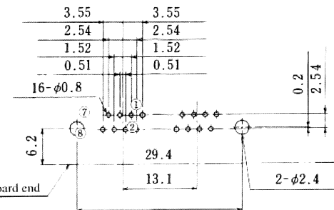
PCB mounting hole layout (Connector mounting side)
