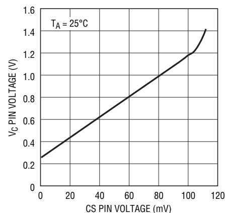
CS Pin to V_C Pin Transfer Function
