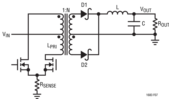
Figure 7. Push-Pull Topology
