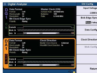
Figure 1: Configure your digital generator DSI settings, including the output format of your choice. Choose amongst four formats: PS, Left Justified, Right Justified and DSP.
