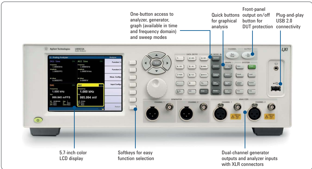
Figure 7. U8903A audio analyzer, front view
