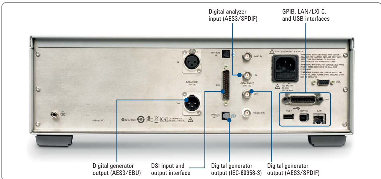
Figure 8. U8903A audio analyzer, rear view
