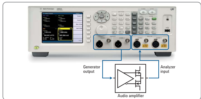
Figure 9. Audio testing using the U8903A.
