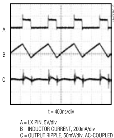
LIGHT-LOAD SWITCHING WAVEFORMS
