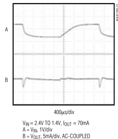
LINE-TRANSIENT RESPONSE
