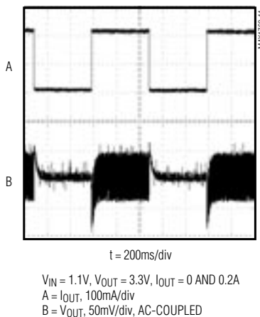
LOAD-TRANSIENT RESPONSE
