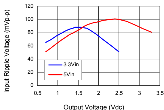
Figure 28. Input ripple voltage for various output with 3x150 μF polymer and 2x47 μF ceramic capacitors at the input (full load)
