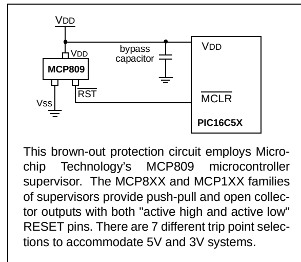
FIGURE 5-8: EXTERNAL BROWN-OUT PROTECTION CIRCUIT 3
