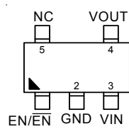
TSOT-23-5/ SOT-23-5(G-Type)
