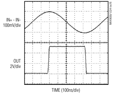
SINUSOID 1MHz RESPONSE AT 1.25MHz V_{OD} = 100mV
