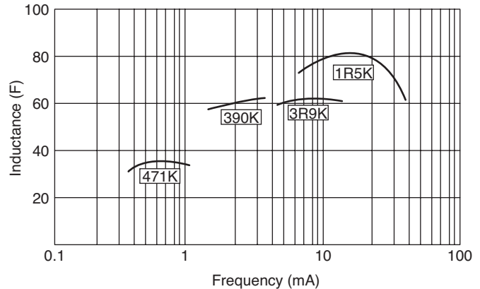
Q-Frequency Characteristics
