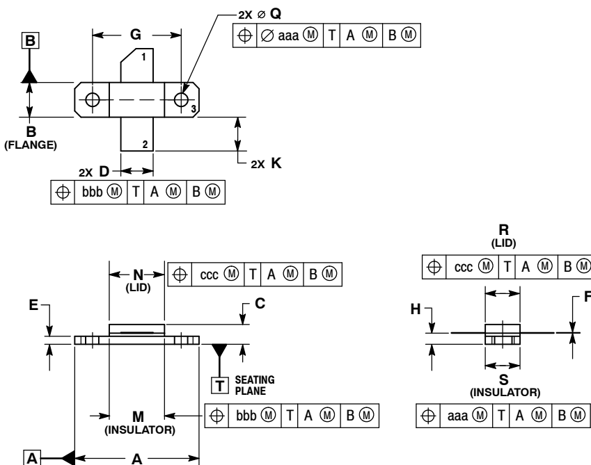
CASE 360B-05 ISSUE G NI-360 MRF21010LR1
