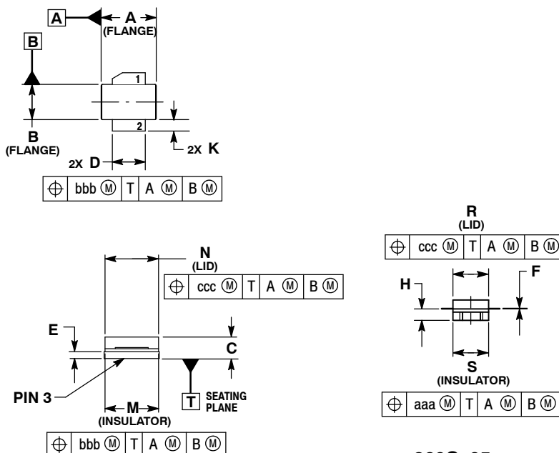
360C-05 ISSUE E NI-360S MRF21010LSR1
