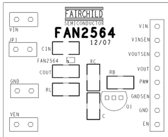
Figure 23. Assembly Diagram
