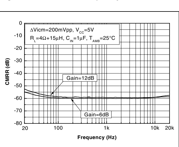
Figure 19. CMRR vs. frequency
