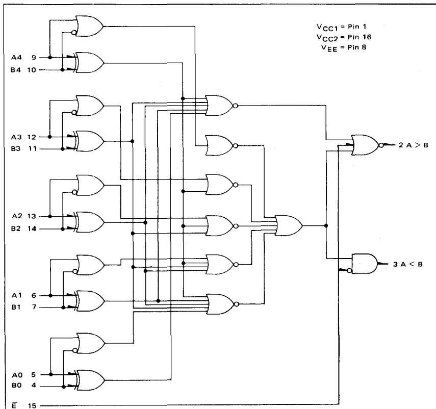
LOGIC DIAGRAM
