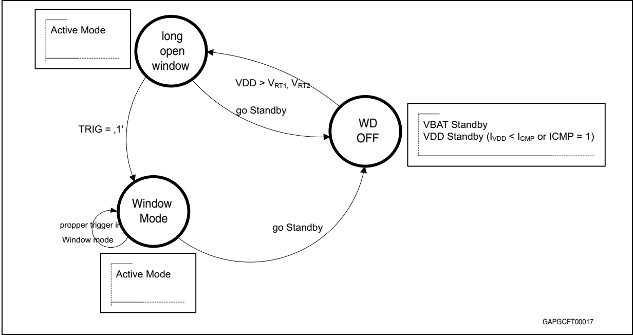
Figure 5. Watchdog in normal operation mode (part 2)
