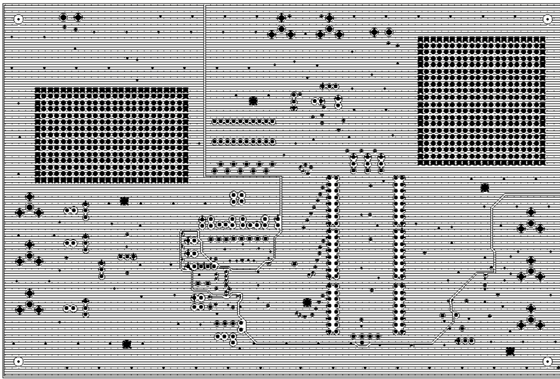
FIGURE 6. ANALOG AND DIGITAL GROUND PLANE
