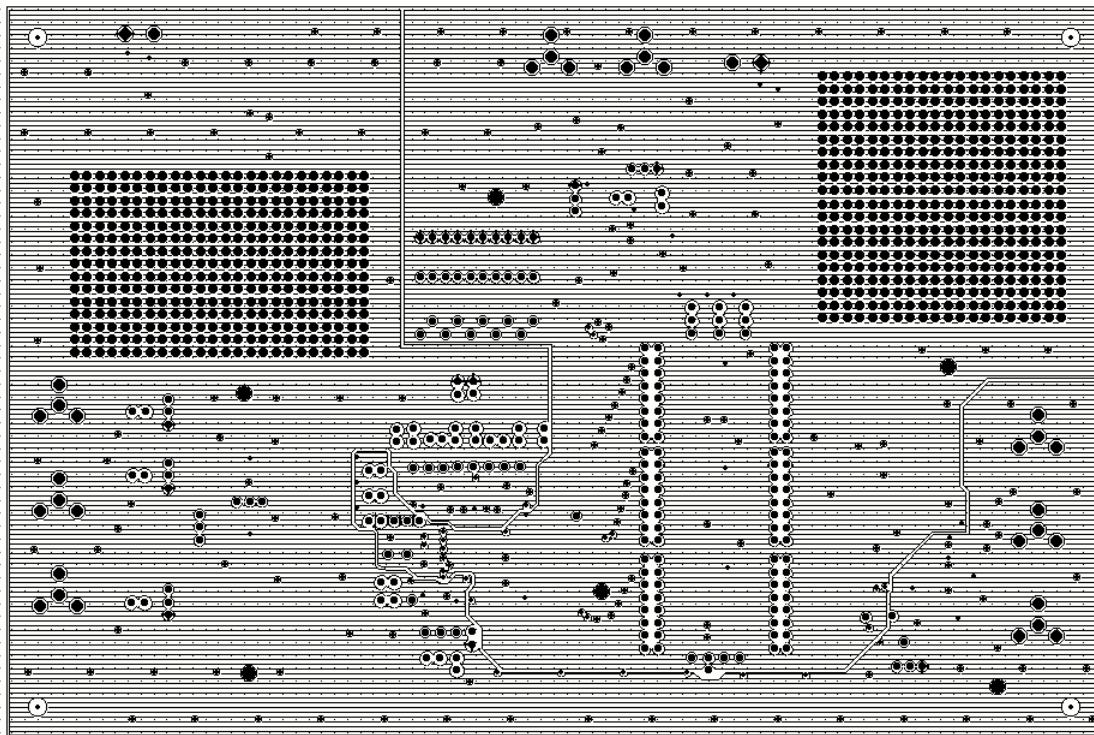
FIGURE 7. ANALOG AND DIGITAL POWER PLANE
