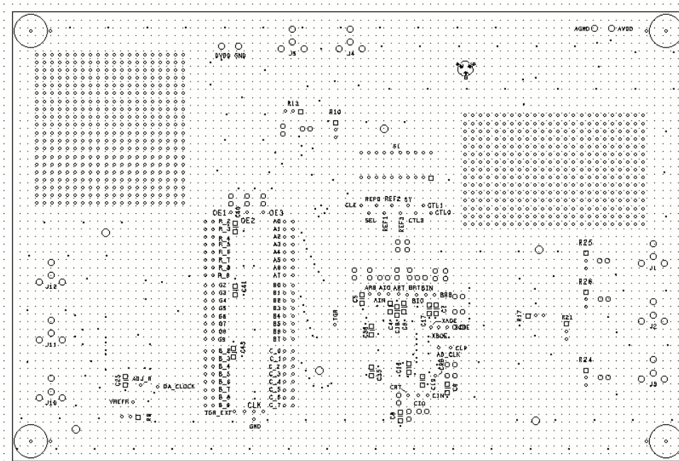
FIGURE 9. BOTTOM SILKSCREEN
