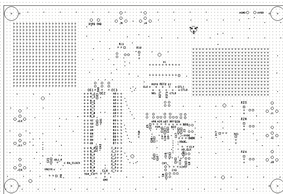
FIGURE 4. TOP SILK SCREEN
