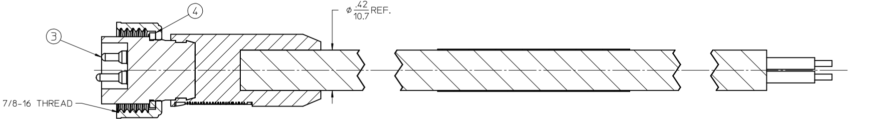
Section Z-Z
