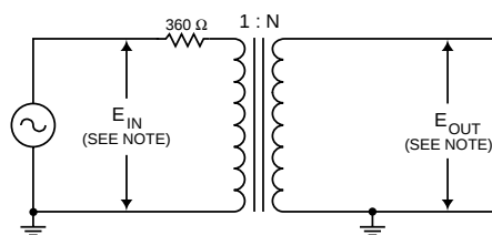
FIGURE 2. CIRCUIT FOR COMMON-MODE REJECTION
