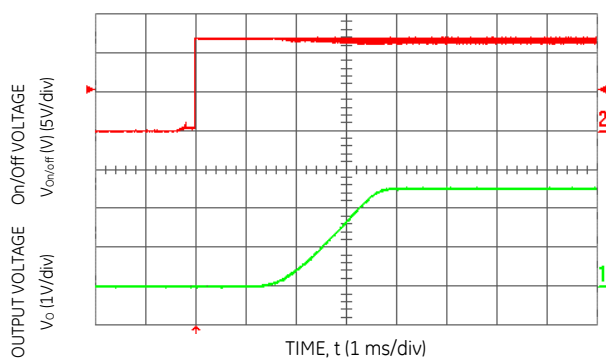
Figure 15. Typical Start-Up Using Remote On/Off with Low-ESR external capacitors ( C_o = 5000 \mu F) ( V_{in} = 12.0 Vdc, V_o = 5.0 Vdc, I_o = 10.0 A, C_o = 1050 \mu F).
