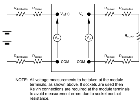
Figure 25. Output Voltage and Efficiency Test Setup.
