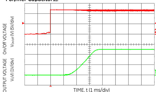
Figure 14. Typical Start-Up Using Remote On/Off ( V_{in} = 12.0 Vdc, V_o = 5.0 Vdc, I_o = 10.0 A).
