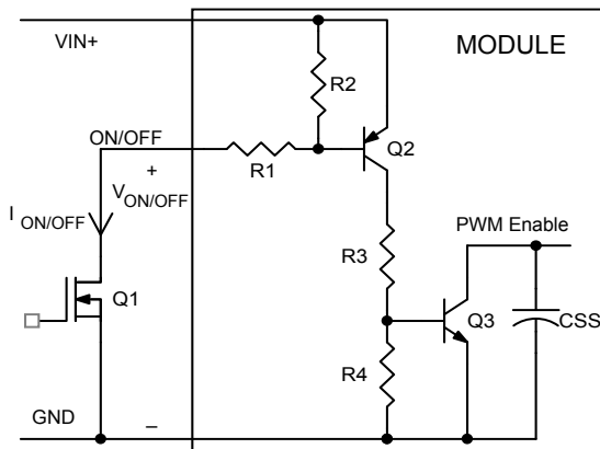
Figure 27. Remote On/Off Implementation.
