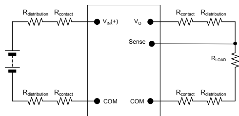
Figure 29. Remote sense circuit configuration
