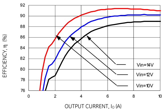
Figure 3. Converter Efficiency versus Output Current (Vout = 1.8Vdc).
