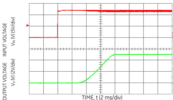
Figure 16. Typical Start-Up with application of V_{in} with low-ESR polymer capacitors at the output ( 7 \times 150 \mu F) ( V_{in} = 12 Vdc, V_o = 5.0 Vdc, I_o = 10 A, C_o = 1050 \mu F).
