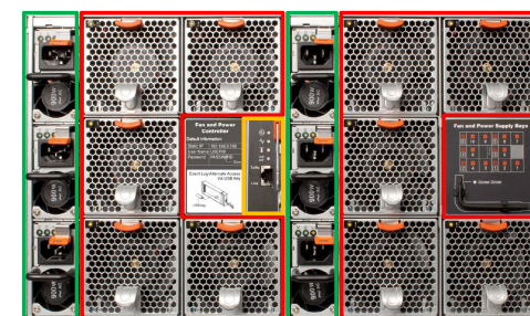
6x Power supplies Fan and Power Controller 10x Fan Modules
