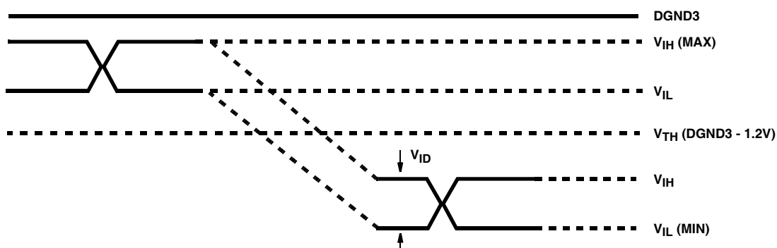
FIGURE 3. ECL AND PECL SWITCHING LEVEL
