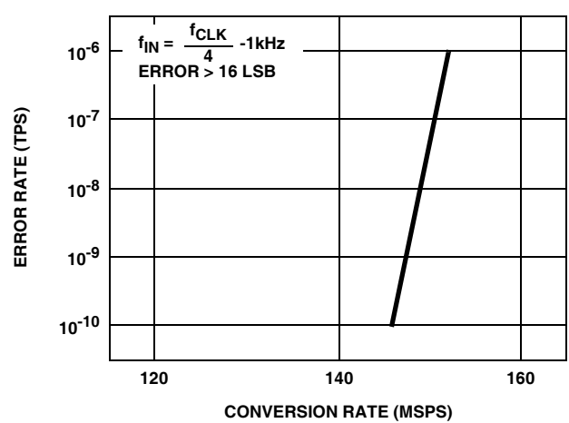
FIGURE 16. ERROR RATE vs CONVERSION RATE CHARACTERISTICS
