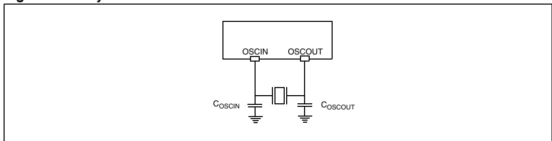
Figure 14. Crystal resonator
