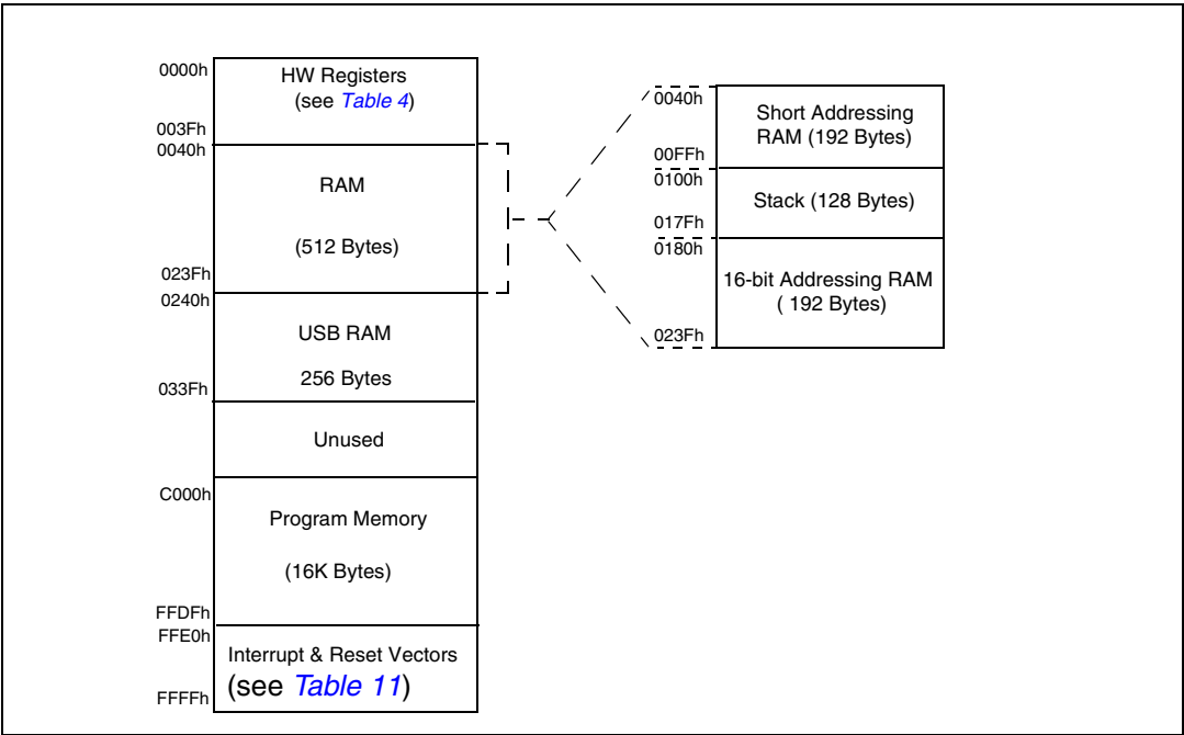
Figure 7. Memory map
