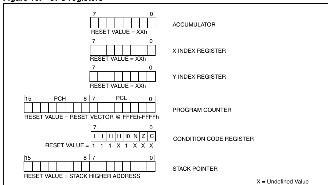
Figure 10. CPU registers
