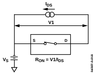
Figure 18. On Resistance
