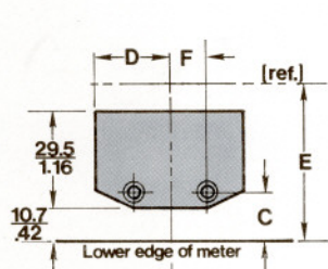
8S and 8W barrel detail
