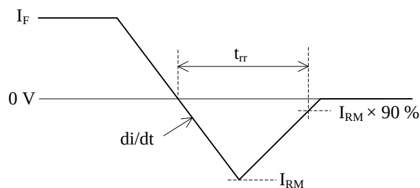
(b) Waveform
