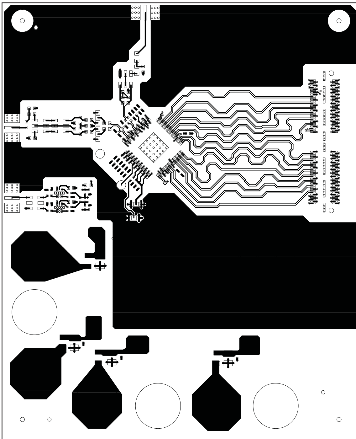
Figure 4. Component Side
