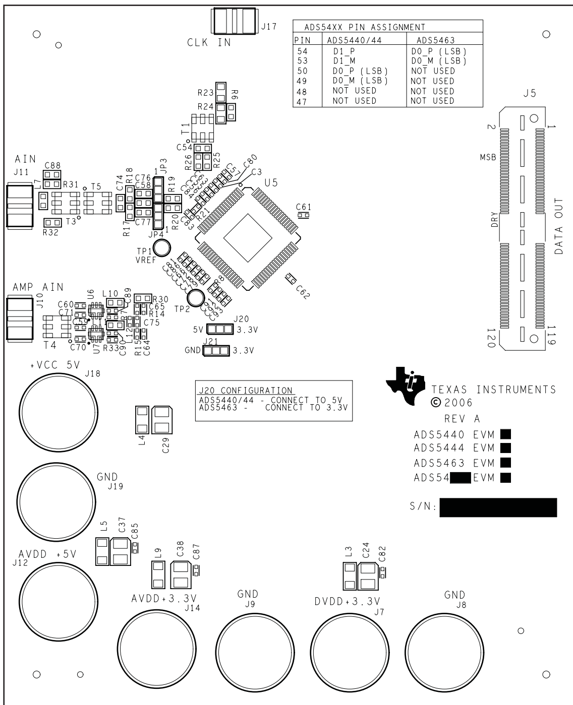
Figure 3. Top Silkscreen
