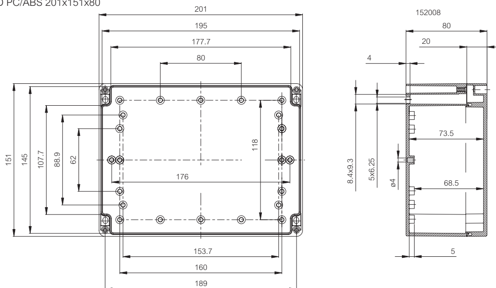
EURONORD PC/ABS 201x151x80
