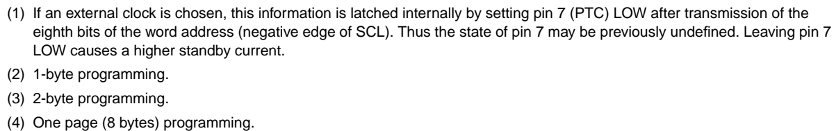
Fig 13. External clock.
