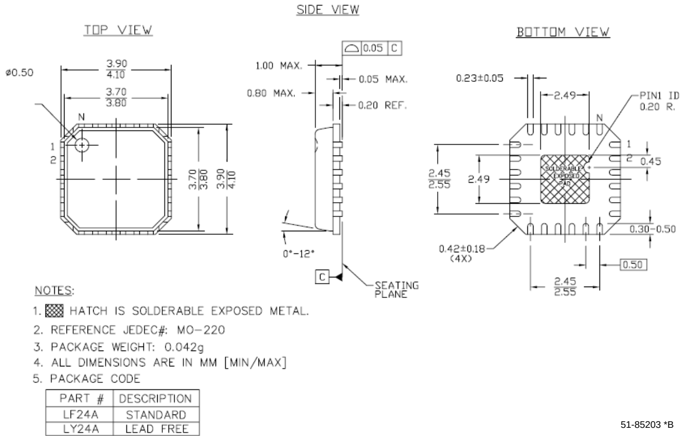
Figure 14. 24-Pin (4x4) QFN
