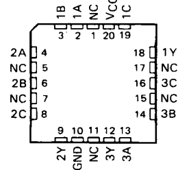
SN54ALS15A . . . FK PACKAGE (TOP VIEW)
