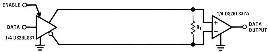
Two-Wire Balanced Interface—RS-422
