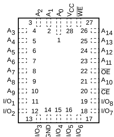
28 LCC (L5)
