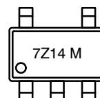
SOT23-5 CASE 527AH
