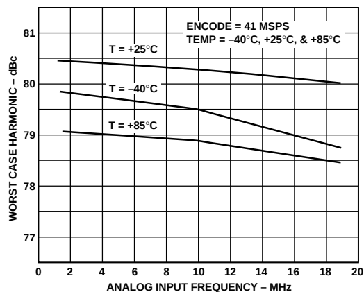
Figure 11. Harmonics vs. AIN
