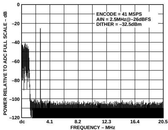
Figure 25. 128K FFT with Dither
