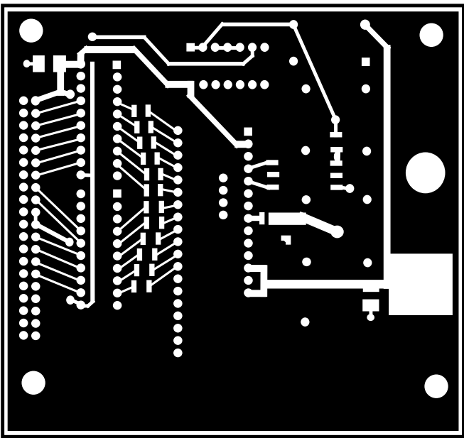
Figure 42. AD9042D/PCB Bottom Side Copper (Negative)
