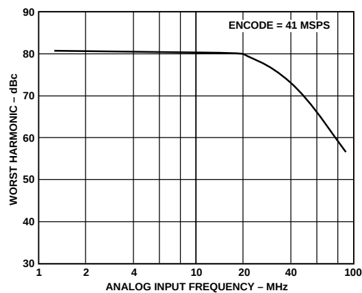
Figure 13. Harmonics vs. AIN
