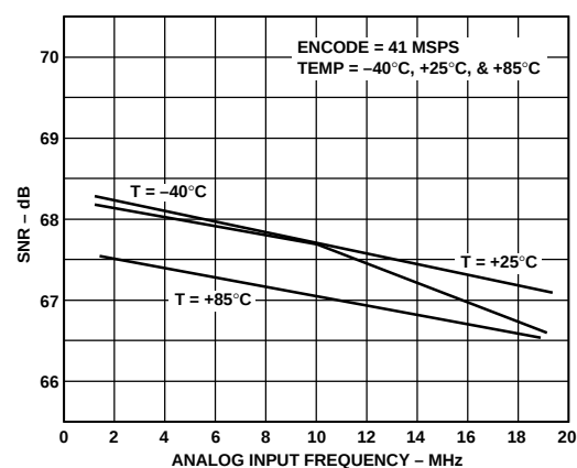
Figure 12. Noise vs. AIN
