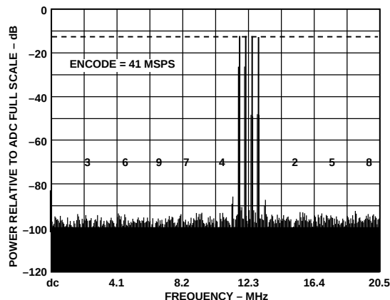
Figure 56. Multitone Performance
