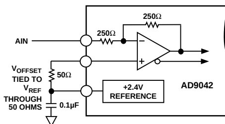
Figure 33. Analog Input Offset by +2.4 V Reference
