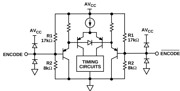
Figure 3. Encode Inputs
