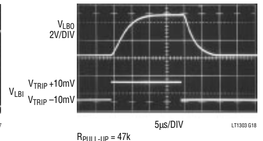
Low Battery Detector Transient Response
