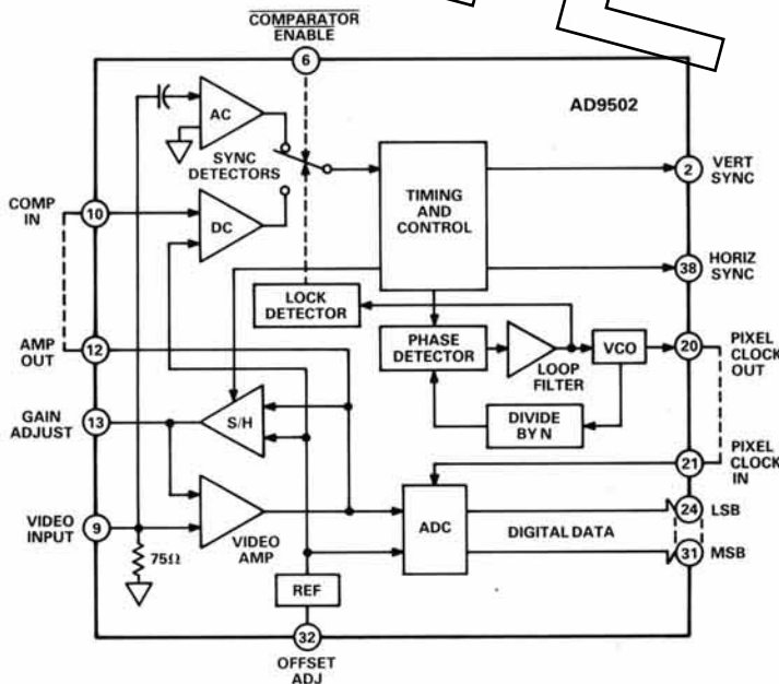
AD9502 Functional Block Diagram
