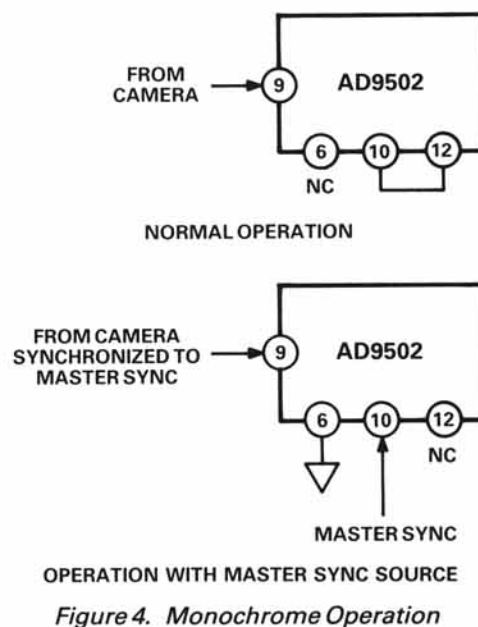
Figure 4. Monochrome Operation
