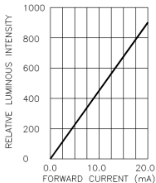
Forward Current vs. Relative Luminous Intensity
